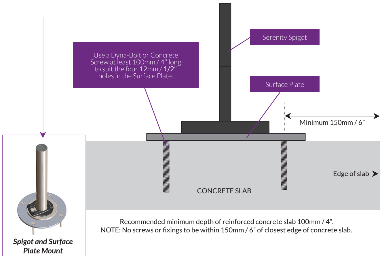
Figure J - Securing Surface Plate to Concrete Slab
