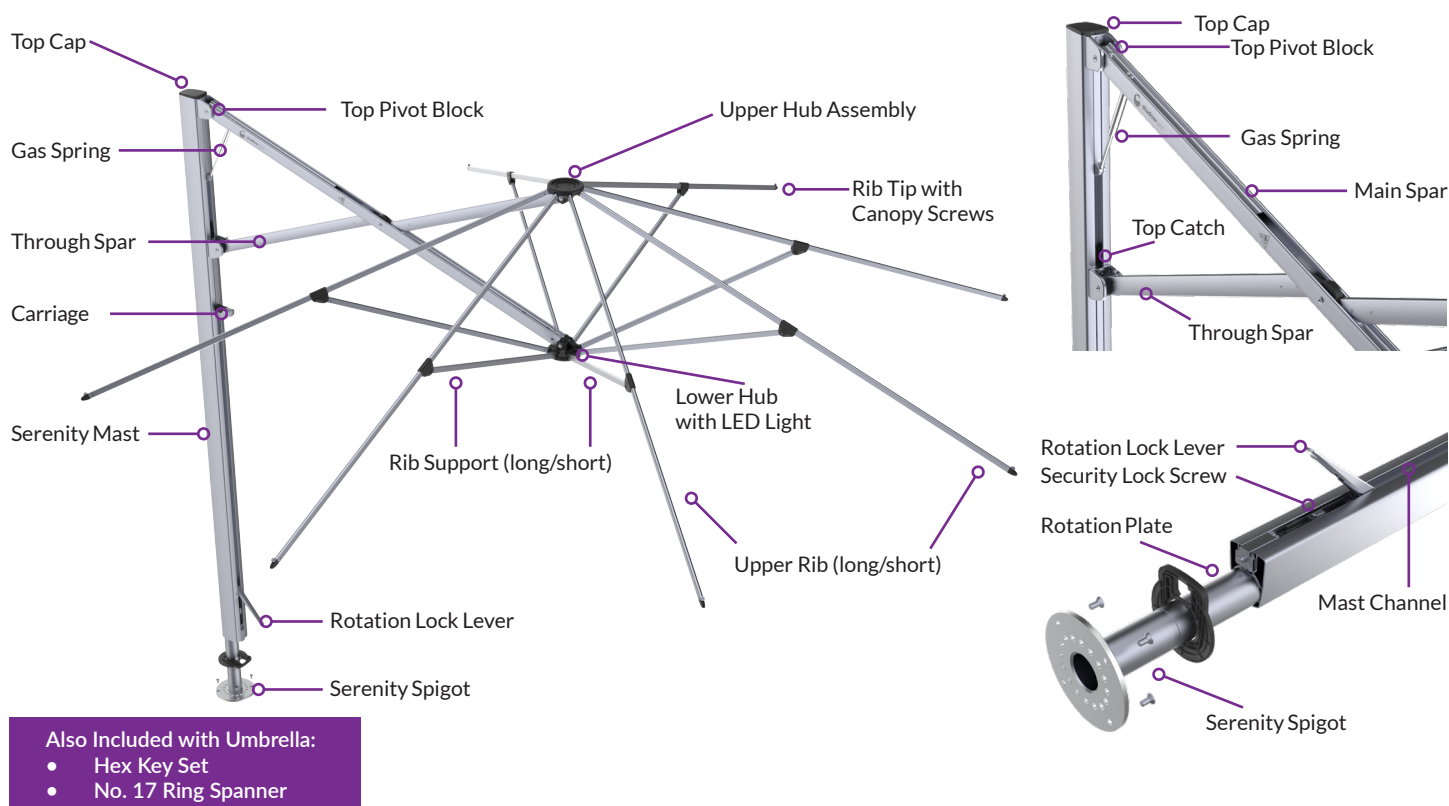
Figure B - Serenity Umbrella Parts
