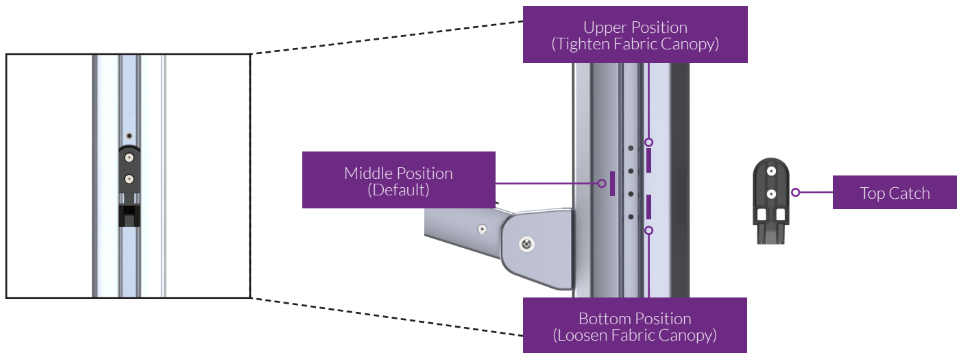
Figure N - Top Catch Permanent Operational Position
