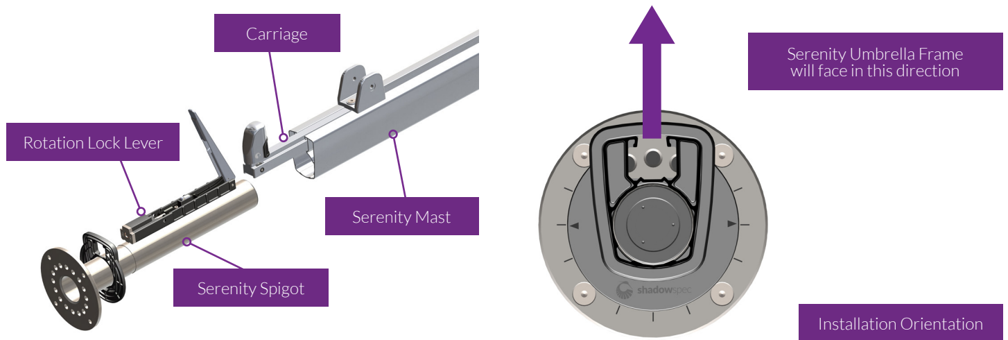
Figure M - Carriage and Rotation Lock Lever Assembly
